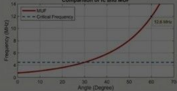
Comparison of f_c and MUF
