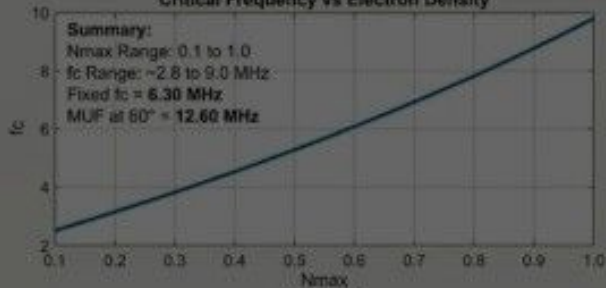
Critical Frequency vs Electron Density
